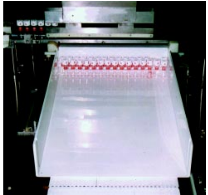
Model 229008 Vial Loading Tray
